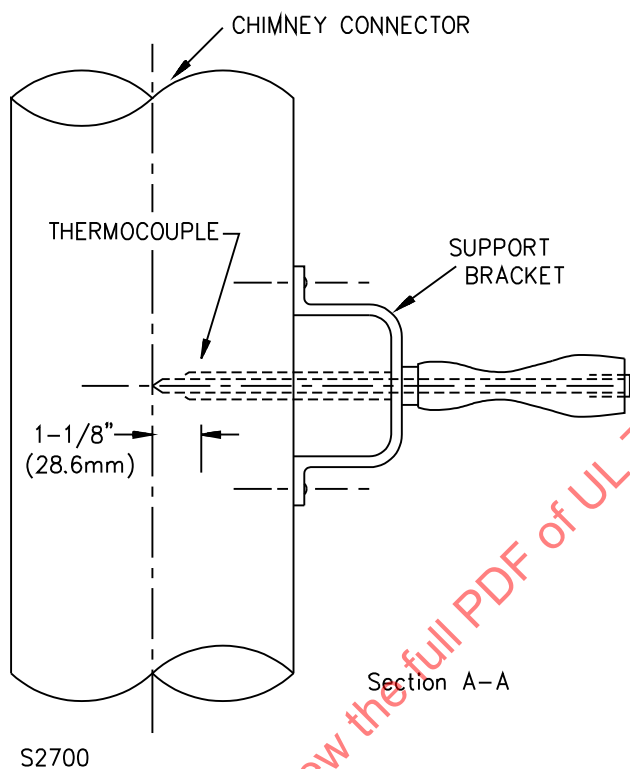
Figure 39.2 Flue Gas Thermocouple and Support Bracket
