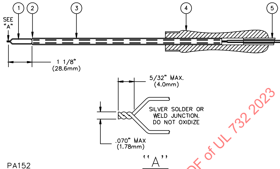
Figure 39.1 Standard Thermocouple for Flue-Gas Temperature
