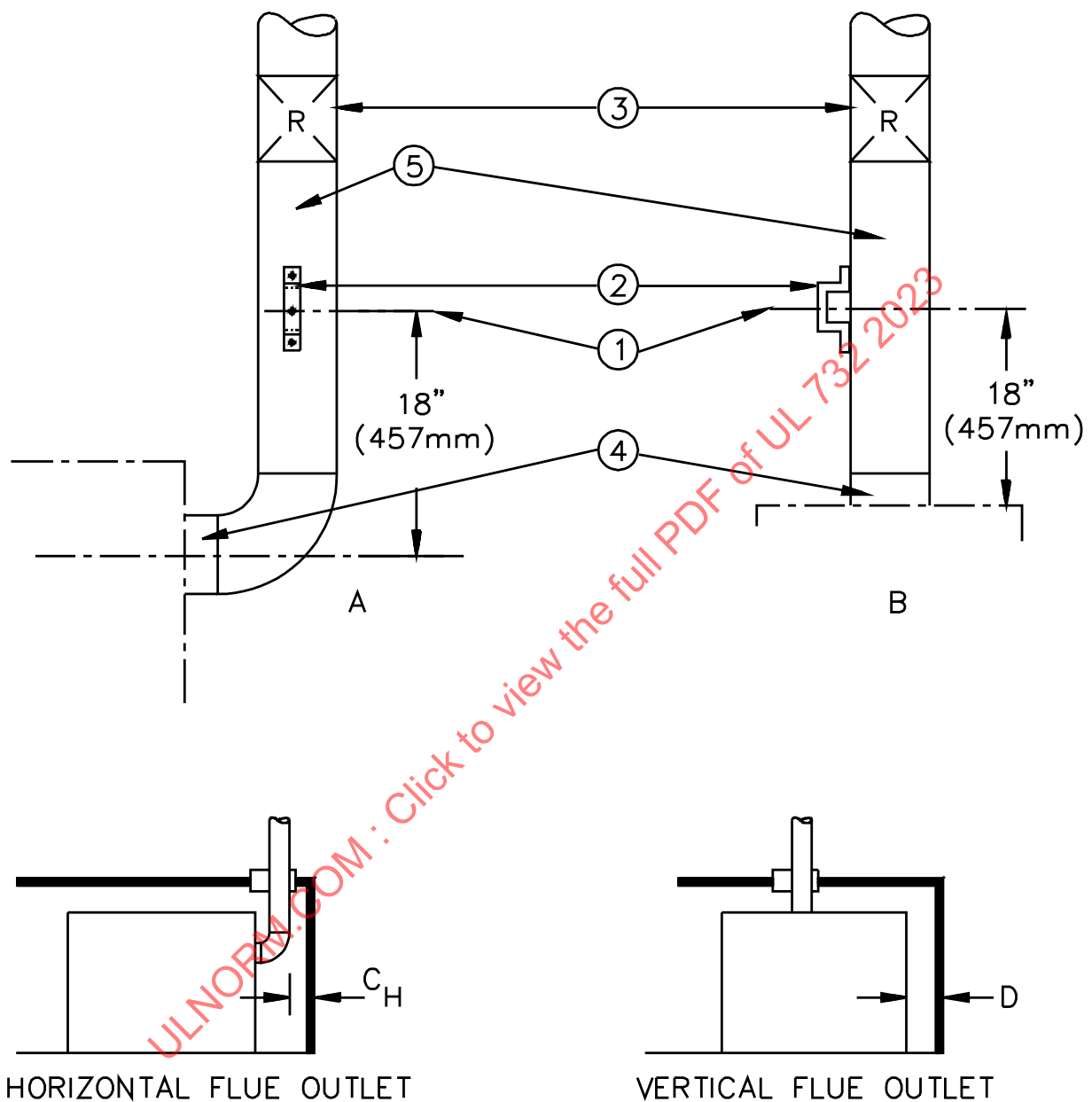
Figure 37.2 Chimney Connector – Standard Clearance Test
