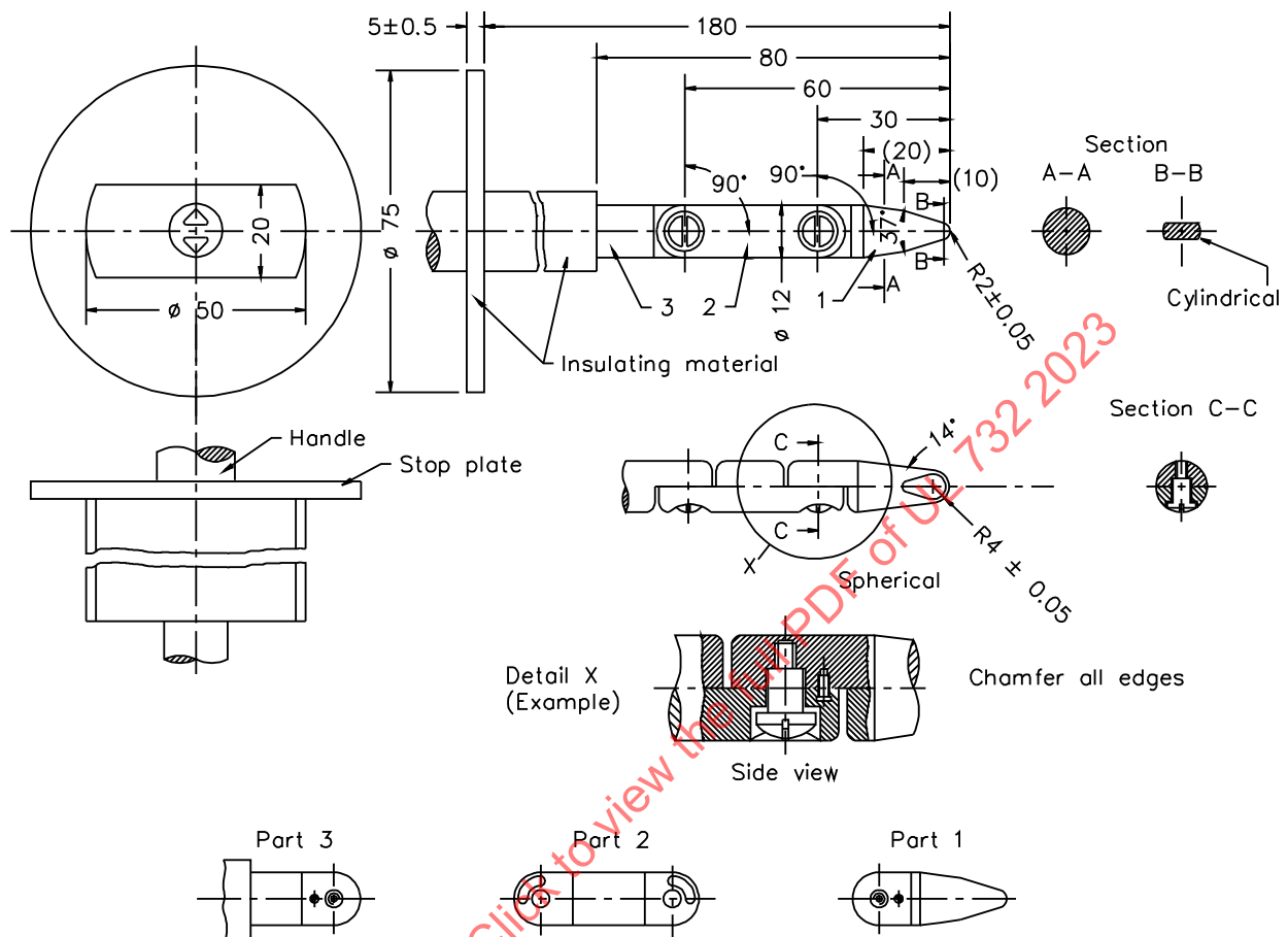
Figure 28.4 IEC Articulate Probe
