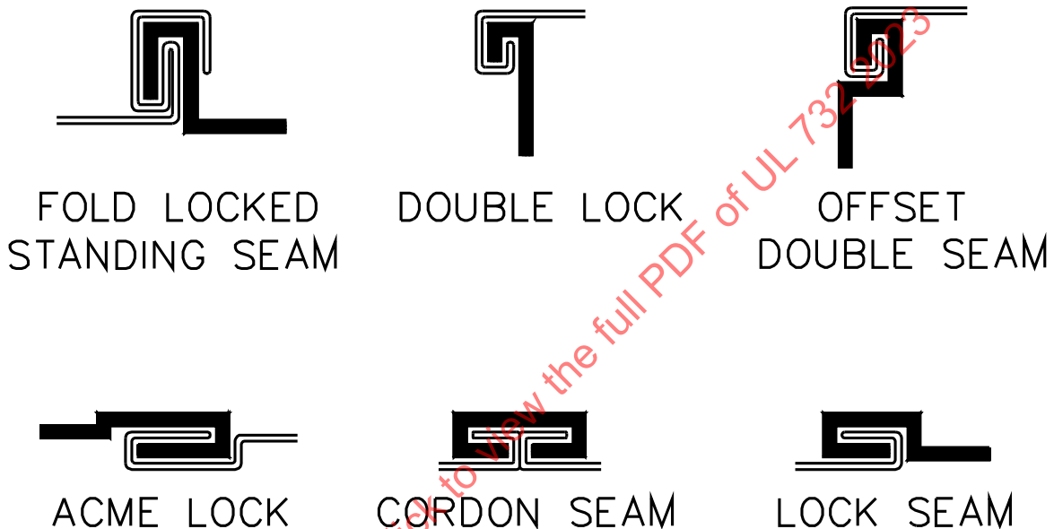
Figure 13.1 Types of Acceptable Lock-Seams
