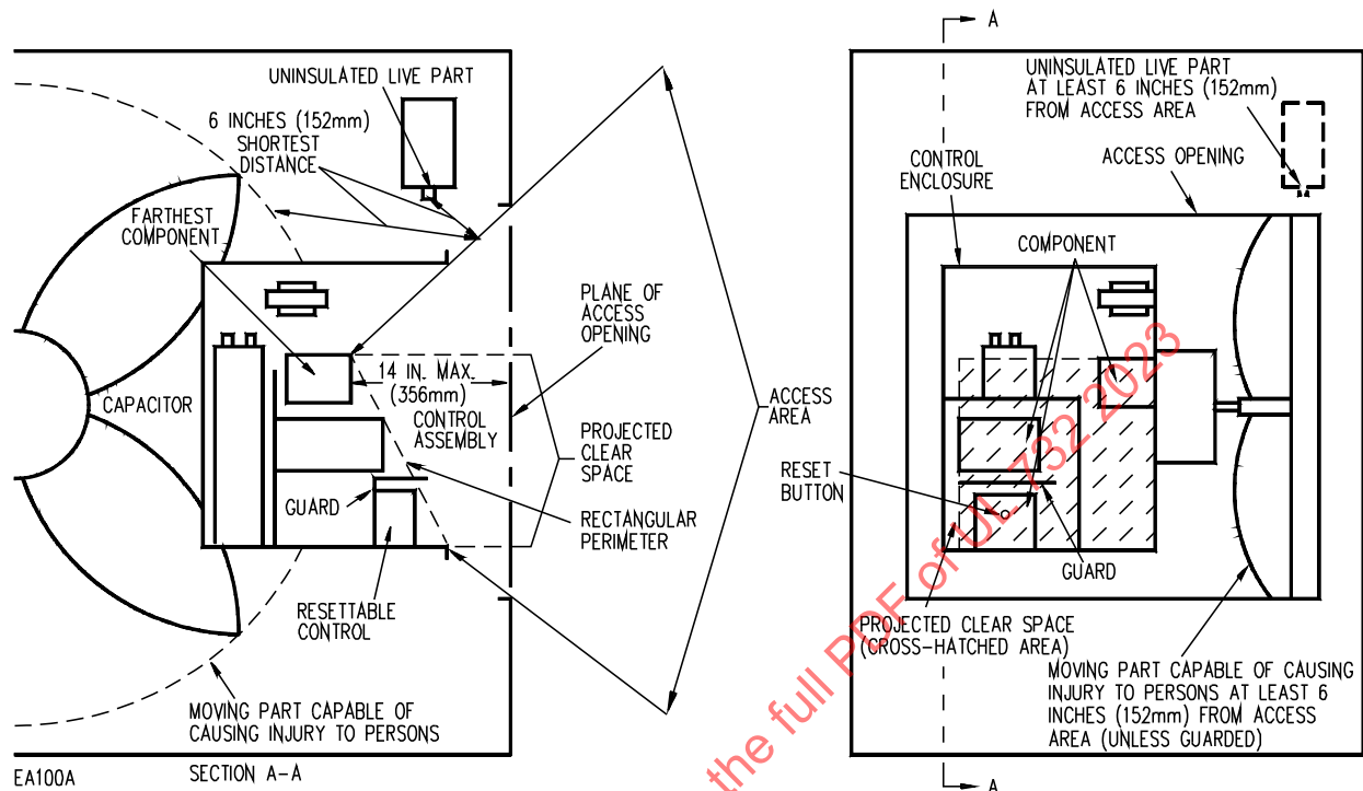
Figure 35.1 Accessibility and Protection
