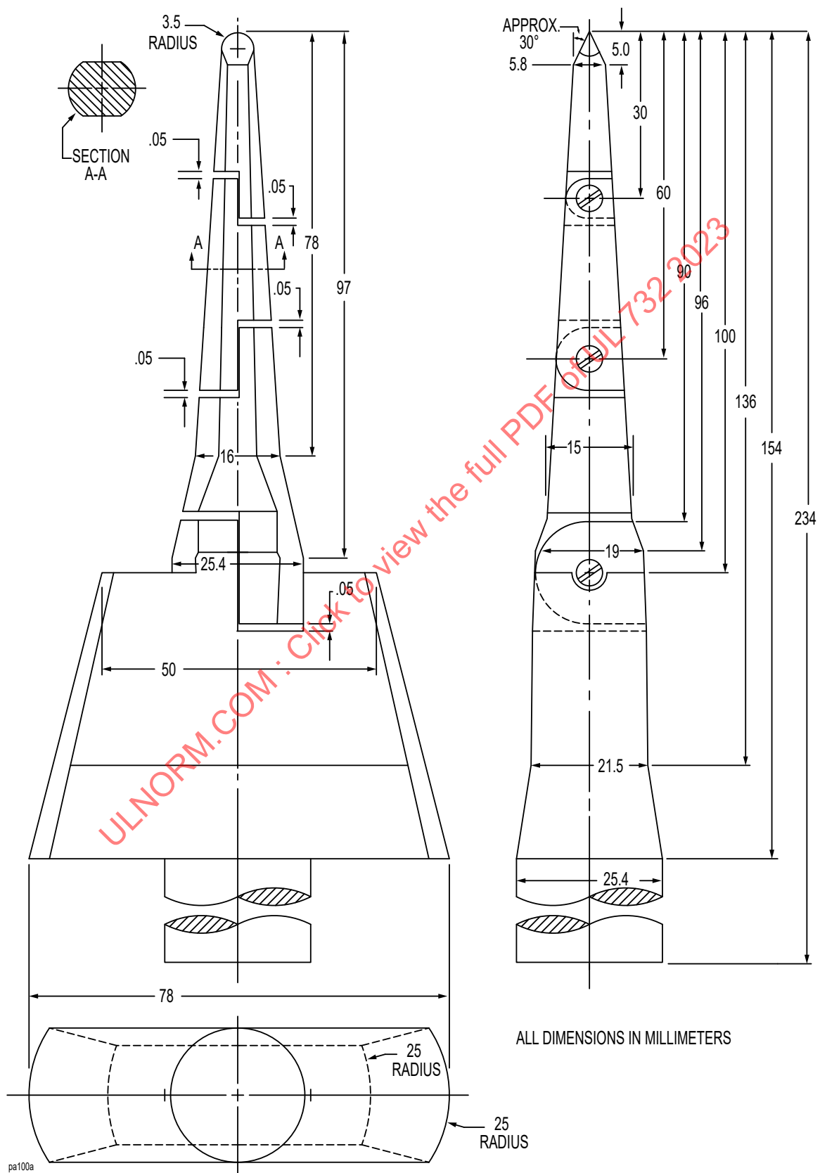
Figure 28.1 Probe for Uninsulated Live Parts
