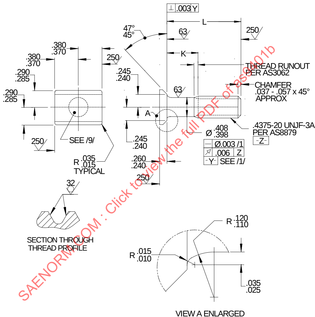
FIGURE 1 - BOLT
