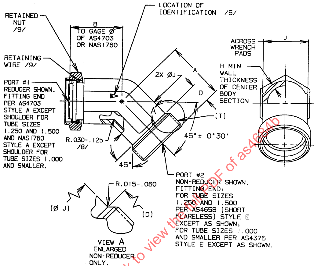
FIGURE 1 - ELBOW ASSEMBLY, 45°
