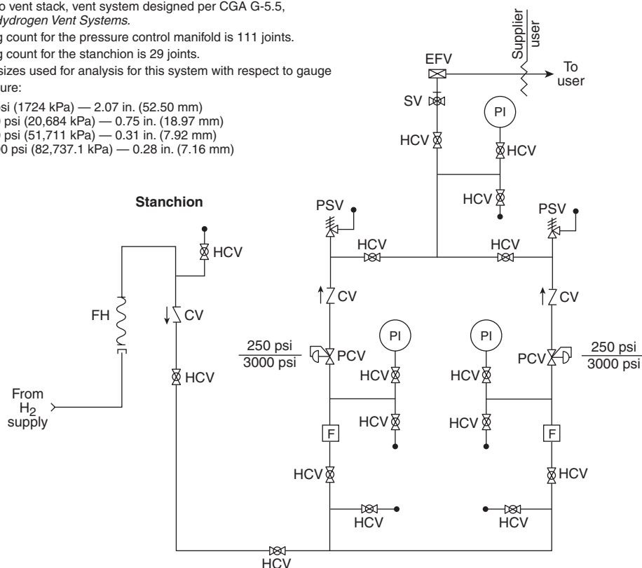
FIGURE A.3.93.2(d) Typical Tube Trailer Discharge Stanchion and Pressure Control Manifold.
