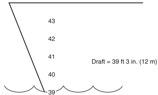
FIGURE 6.10.2.1.1 Draft Marks.
