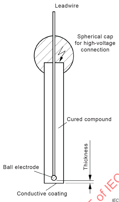
Figure 4 – Example of electrode arrangement for rigid cured compound
