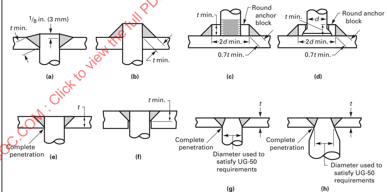
Figure UW-19.1 Typical Forms of Welded Staybolts
