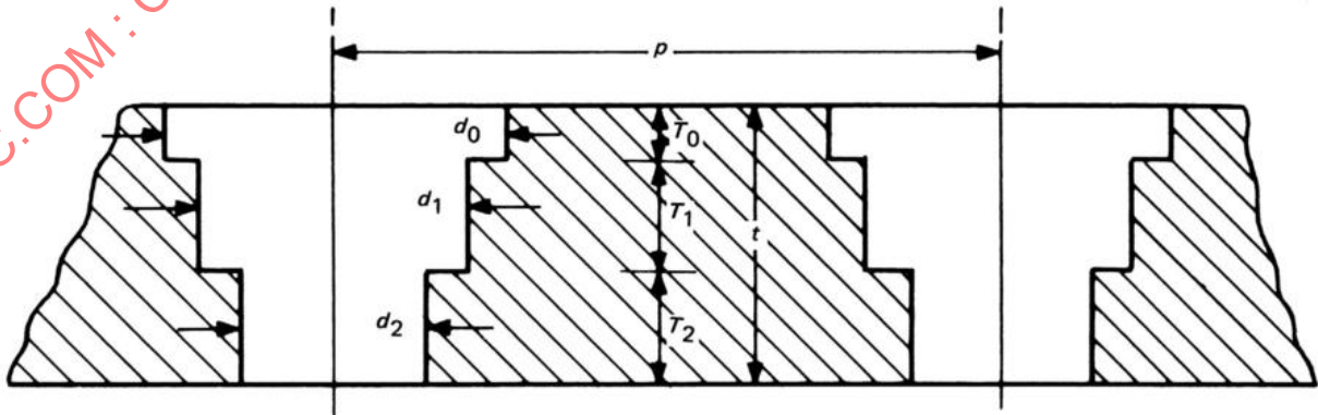
Figure 13-6 Plate With Multidiameter Hole Pattern
