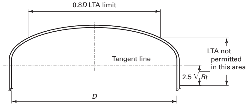
Figure 32-4-2 Limits for Ellipsoidal Head
