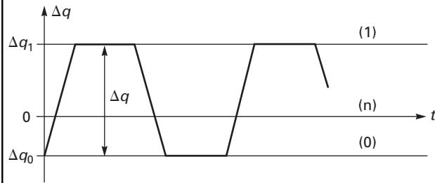
Figure 26-11 Cyclic Displacements
