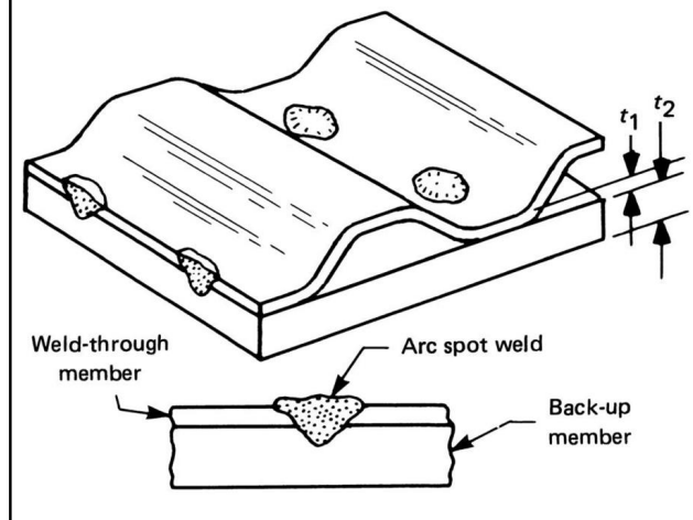
Figure 17-4 Arc-Spot-Welded Two-Layer Assembly
