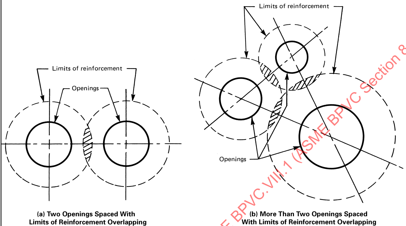
Figure UG-42 Examples of Multiple Openings
