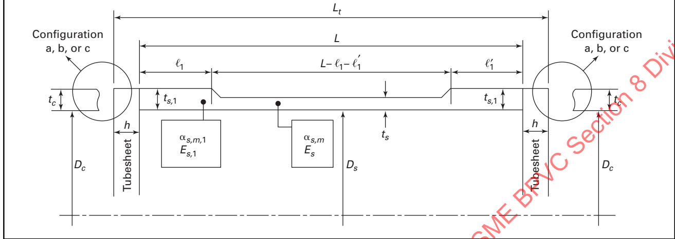
Figure UHX-13.4 Different Shell Thicknesses and/or Material Adjacent to the Tubesheets
