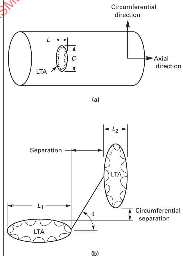
Figure 32-3 Nomenclature
