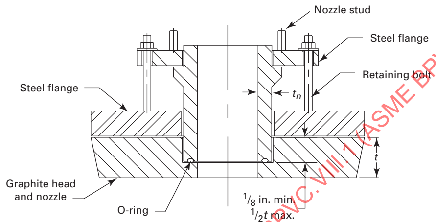
(e) O-Ring
