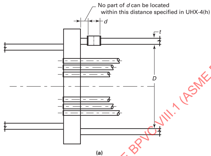
Figure UHX-4-1 Nozzles Adjacent to Tubesheets
