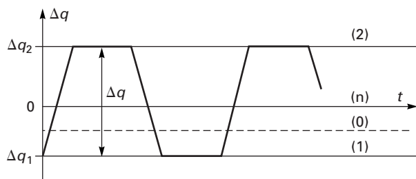
Figure 26-12 Cyclic Displacements
