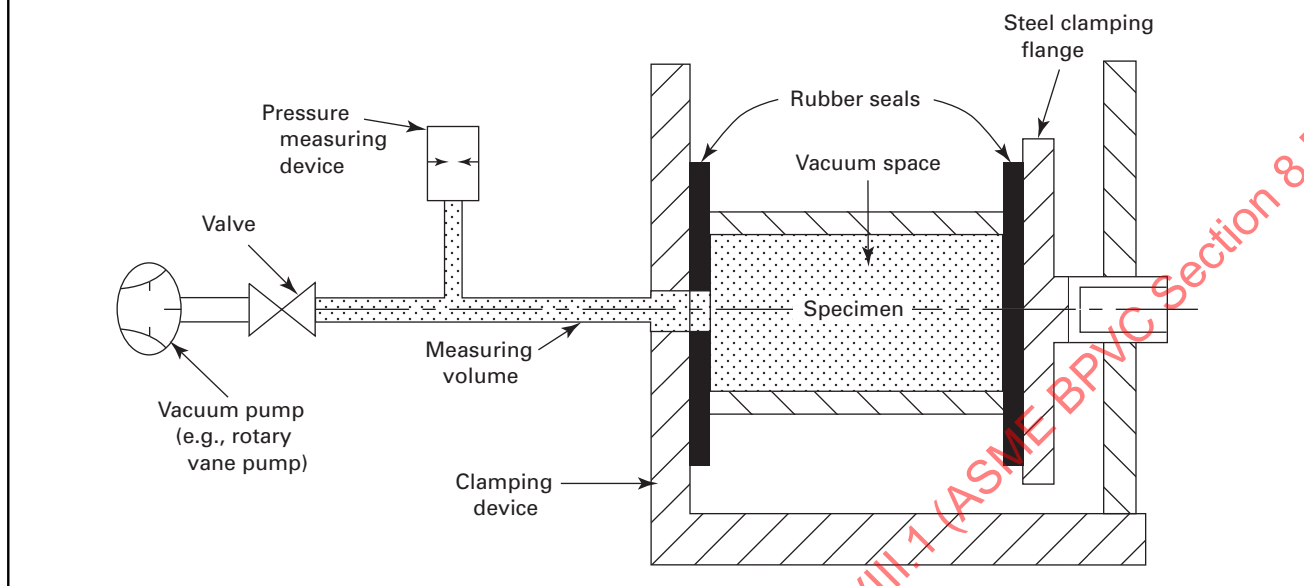
Figure 39-4-1 Schematic Diagram of Vacuum Apparatus
