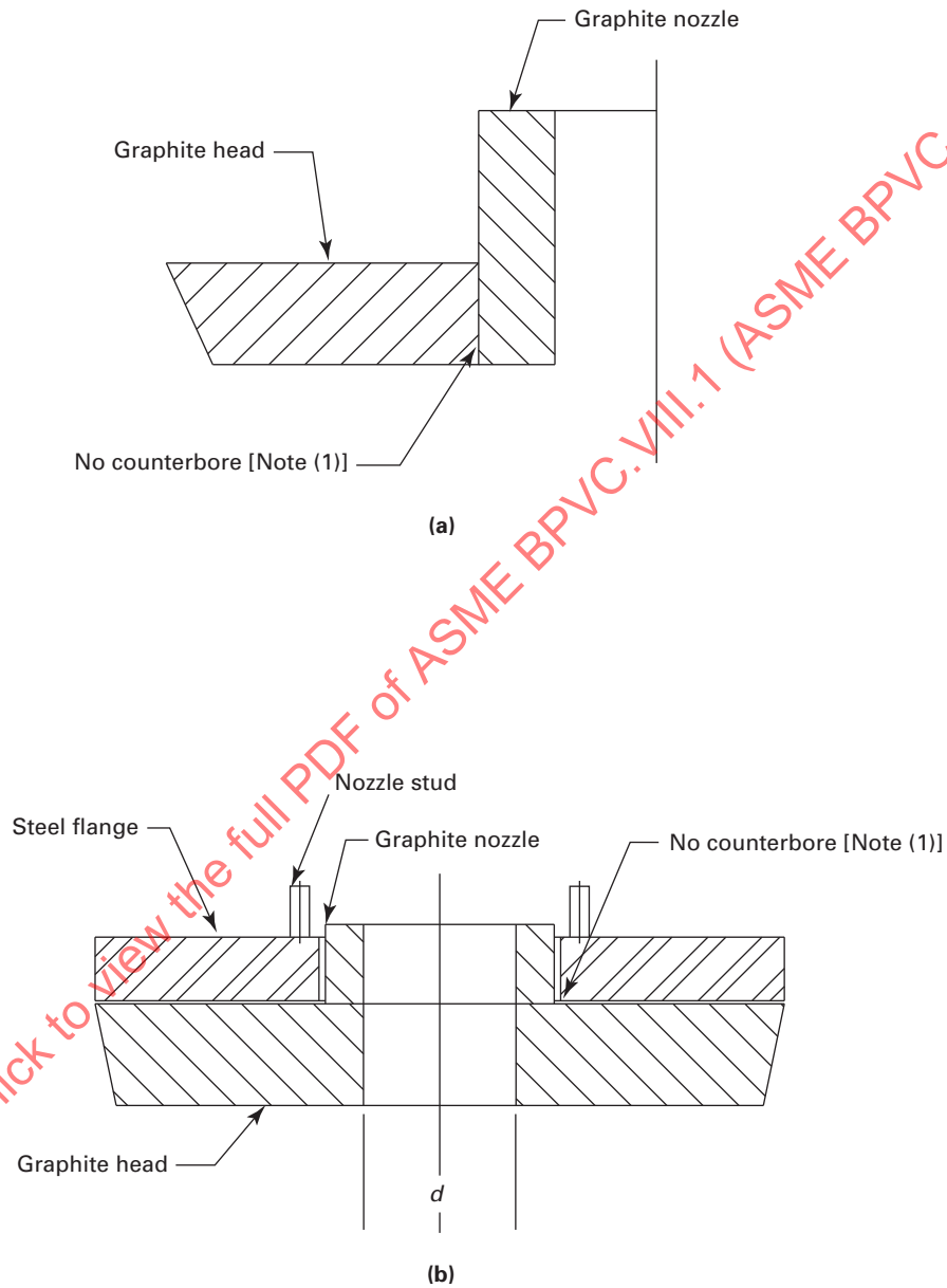
Figure UIG-36-1 Unacceptable Nozzle Attachment Details
