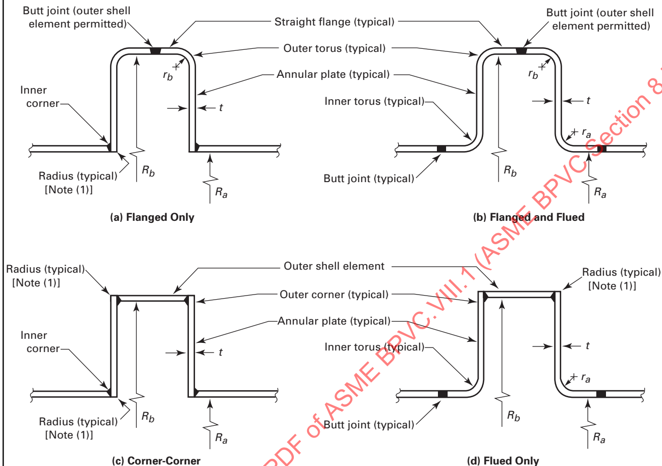
Figure 5-1 Typical Flexible Shell Element Expansion Joints
