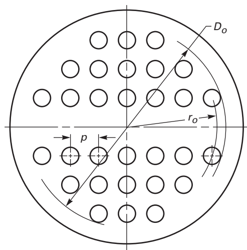
(a) Tubesheet Layout
