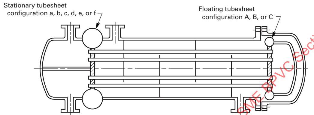
(a) Typical Floating Tubesheet Exchanger With an Immersed Floating Head
