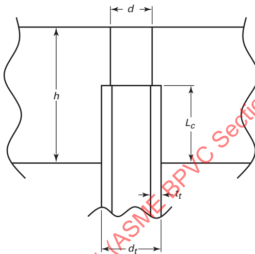
(b) Tube Joint
