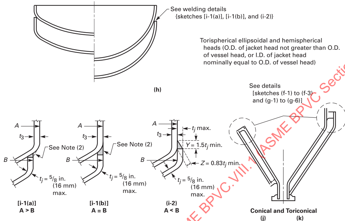
Figure 9-5 Some Acceptable Types of Jacket Closures (Cont'd)
