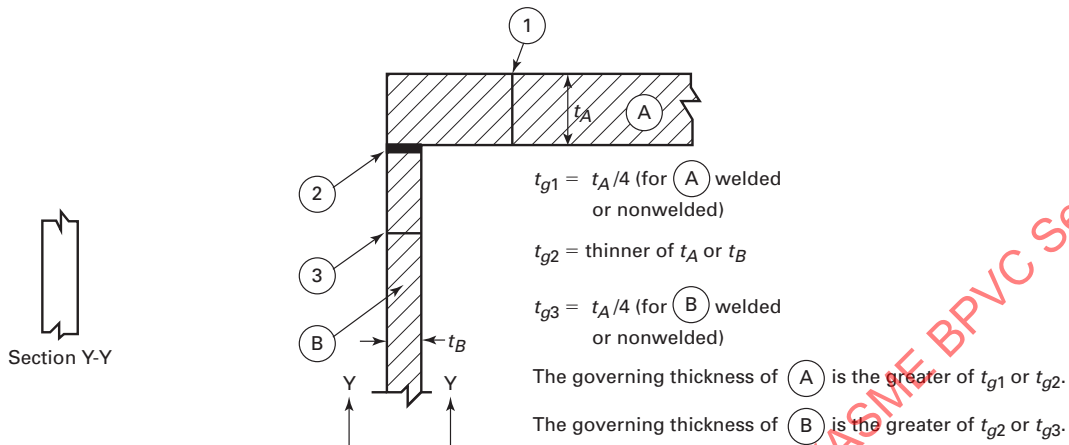
(f) Two Flat Plates With a Corner Joint
