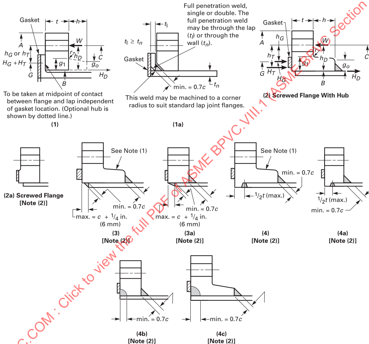
Figure 2-4 Types of Flanges
