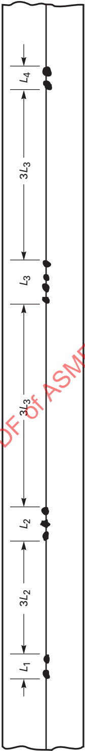
Figure 4-2 Groups of Aligned Rounded Indications
