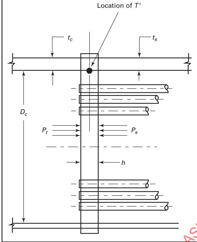
Figure UHX-11.5.1-3 Location of Tubesheet Metal Temperature, T' , at Rim
