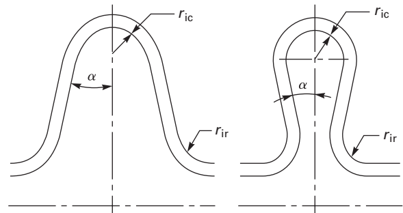
Figure 26-3 Possible Convolution Profile in the Neutral Position
