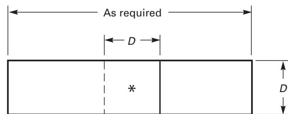
Figure 17-7 Single-Spot-Weld Tension Specimen, Two-Ply Joint
