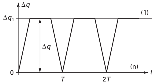
Figure 26-10 Cyclic Displacements
