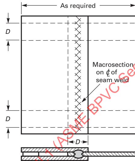
Figure 17-10 Seam-Weld Specimen for Tension and Macrosection for Three-Ply Joint
